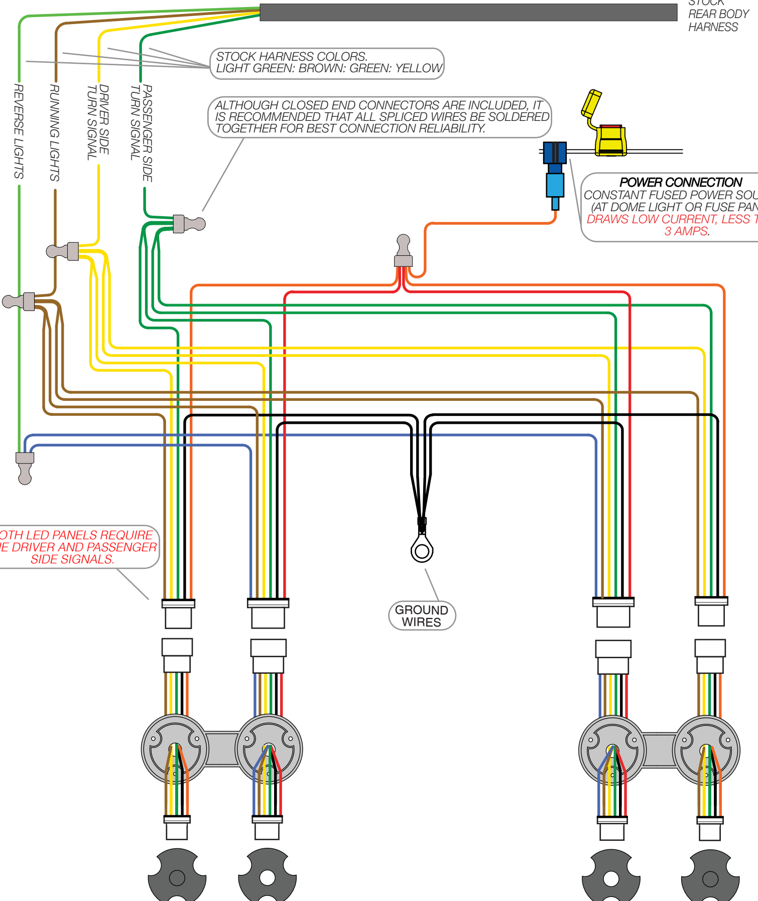
DRIVER SIDE LED PANELS
